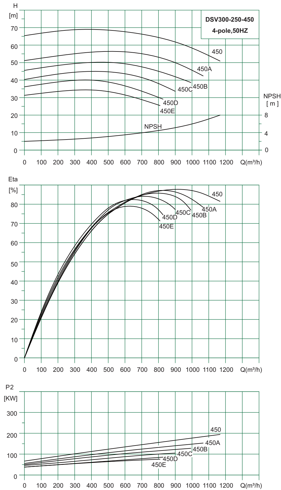
Performance Curve
