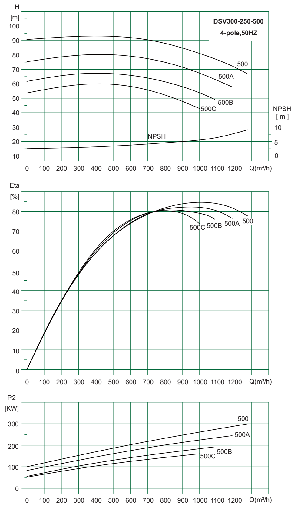
Performance Curve
